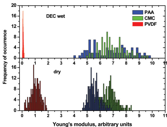
FIGURE 3. Results of AFM stiffness measurements for films made from PAA (100 000 g/mol), CMC, and PVDF. Results are normalized to stiffness of PVDF in dry state.
